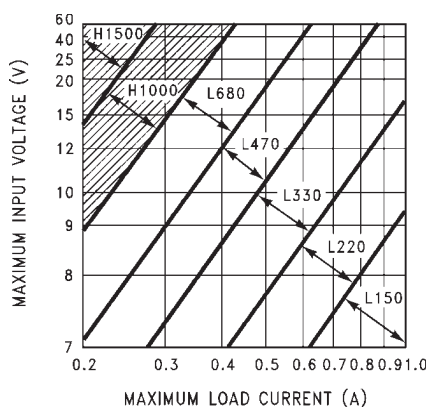
FIGURE 4. LM2575(HV)-5.0
