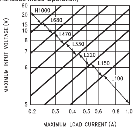
FIGURE 3. LM2575(HV)-3.3
