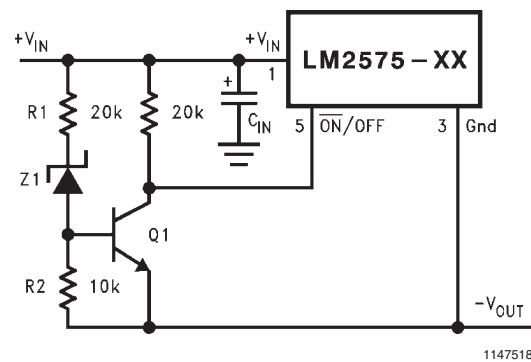
FIGURE 12. Undervoltage Lockout for Buck Circuit
