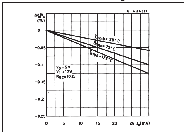
Figure 8. Load regulation characteristics with current limiting
