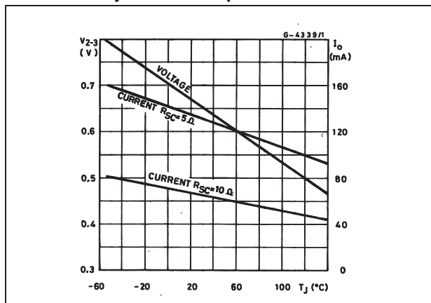
Figure 6. Current limiting characteristics vs junction temperature
