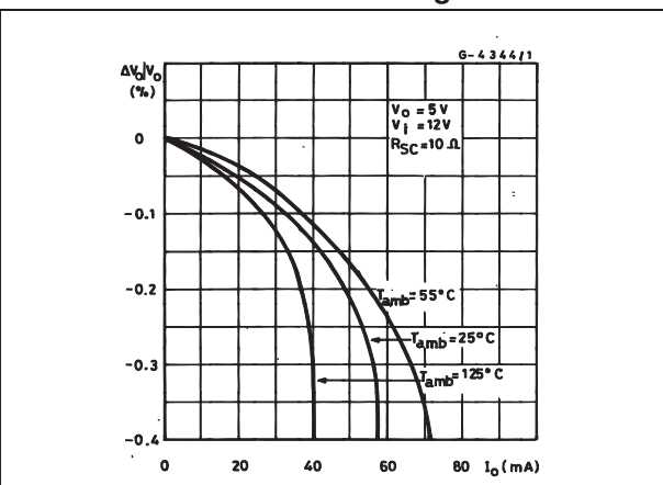
Figure 9. Load regulation characteristics with current limiting
