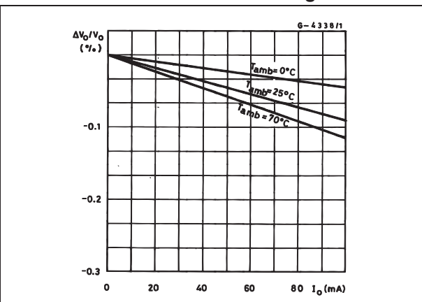
Figure 7. Load regulation characteristics without current limiting
