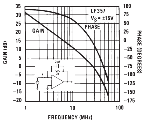
Bode Plot
