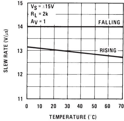
Slew Rate
