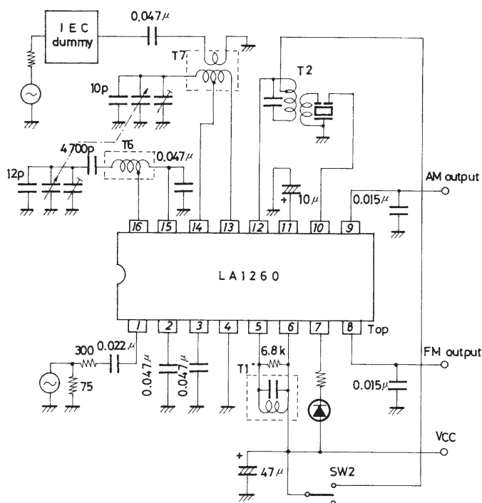
Sample Application Circuit 1 : FM IF/SW2 (7.2 to 24.0MHz)
