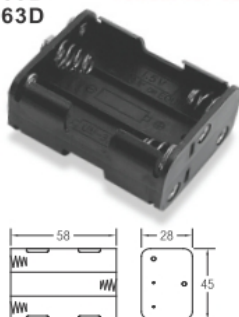
BH363A BH363B BH363D FOR SIX "AA" CELLS
