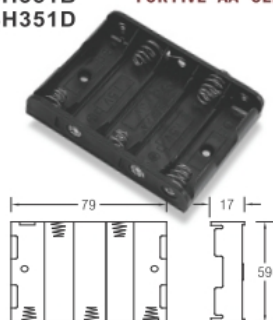
BH351A BH351B BH351D FOR FIVE "AA" CELLS
