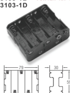
BH3103-1A BH3103-1B BH3103-1D FOR TEN "AA" CELLS
