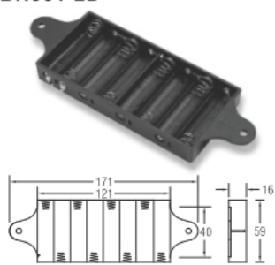
BH381-2A BH381-2B BH381-2D FOR EIGHT "AA" CELLS
