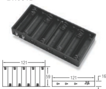
BH381A BH381B BH381D FOR EIGHT "AA" CELLS
