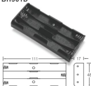
BH361A BH361B BH361D FOR SIX "AA" CELLS
