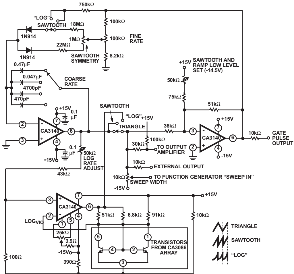
FIGURE 13. SWEEPING GENERATOR
