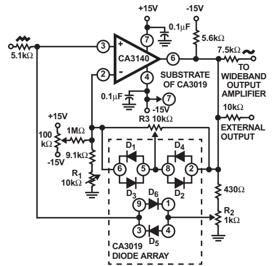
FIGURE 12. SINE WAVE SHAPER
