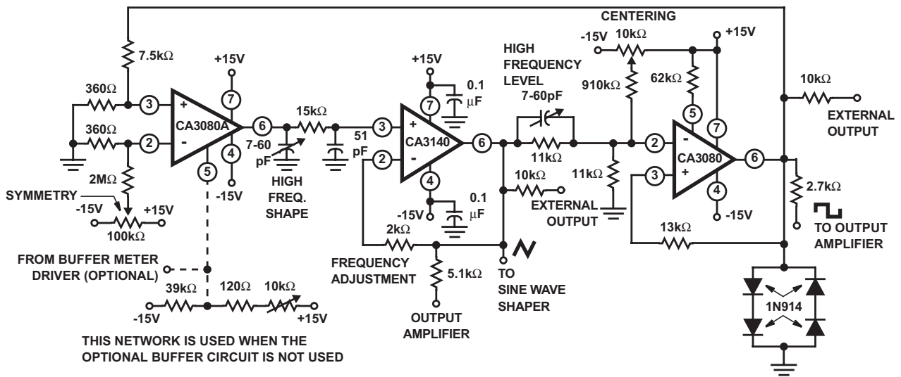
FIGURE 10A. CIRCUIT
