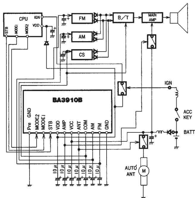
Figure 4 Application example
