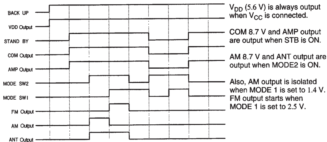
Figure 5 Timing chart
