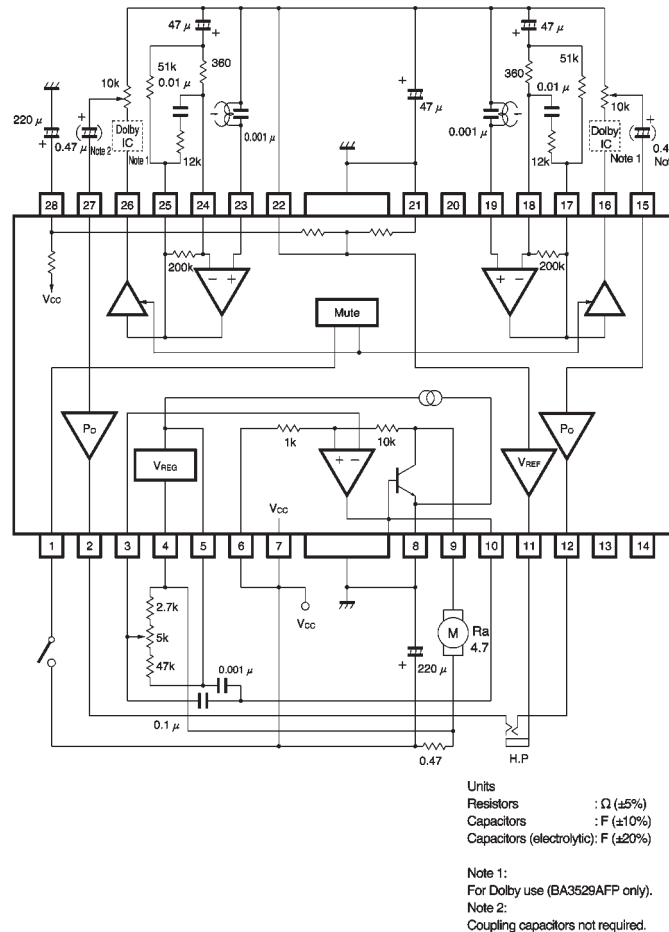
Fig. 7 Headphone stereo with pre-mute
