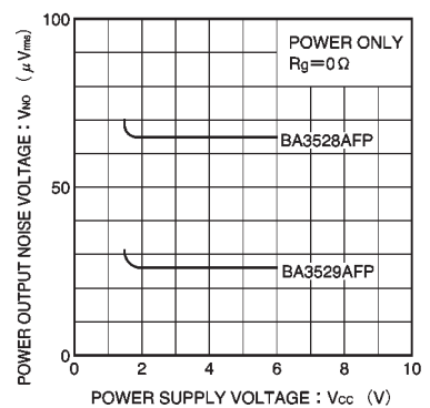
Fig. 26 Output noise voltage vs. power supply voltage
