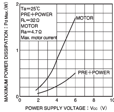
Fig. 19 Maximum power dissipation vs. power supply voltage
