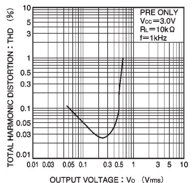
Fig. 23 Total harmonic distortion vs. output voltage
