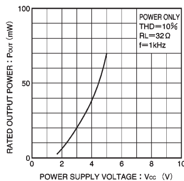
Fig. 25 Rated output power vs. power supply voltage
