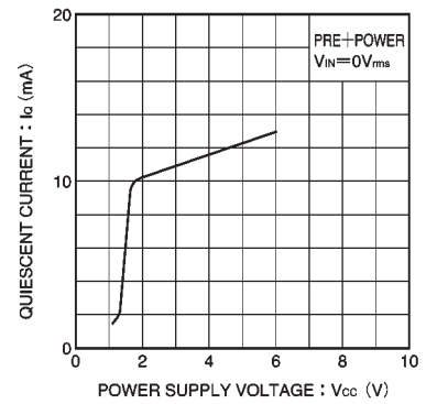
Fig. 20 Quiescent current vs. power supply voltage
