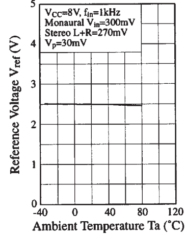
V_{REF} - T_a
