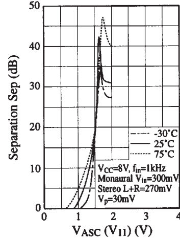
ASC Characteristics
