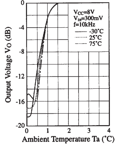
ATC Characteristics
