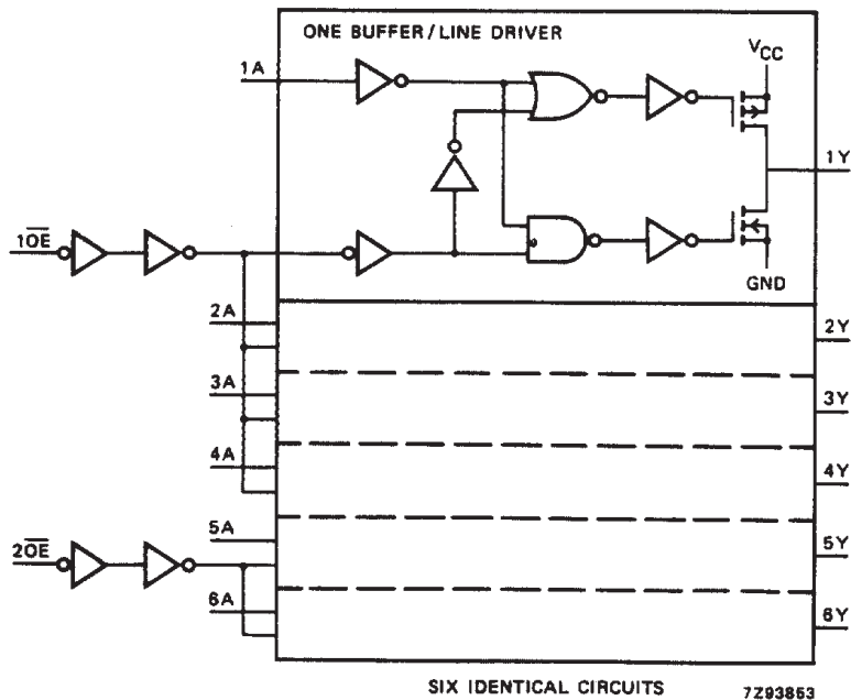
Fig.5 Logic diagram.
