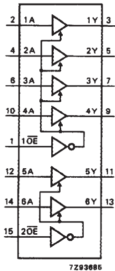
Fig.4 Functional diagram.
