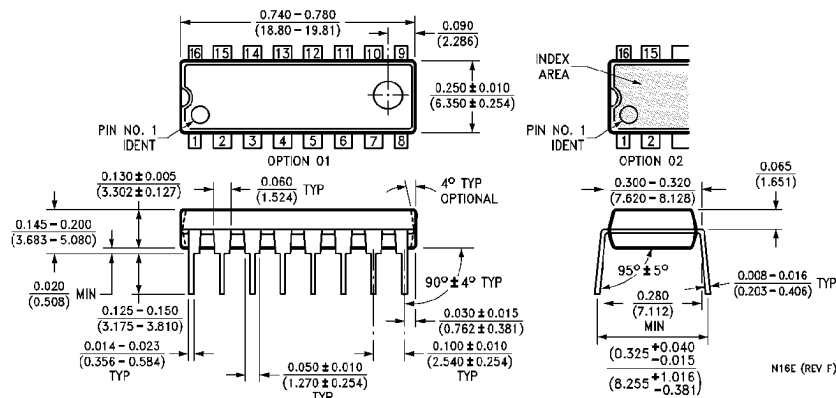
Dual-In Line Package (N) Order Number MM74HC174N See NS Package N16E
