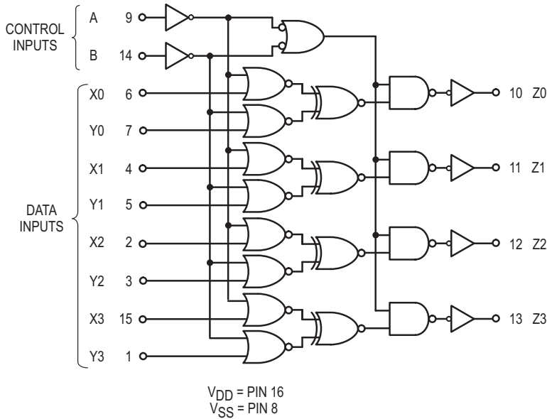
LOGIC DIAGRAM
