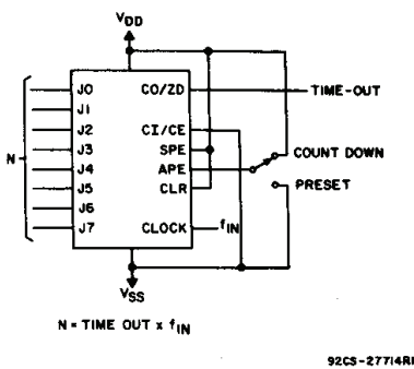
Fig. 19 - Programmable timer.
