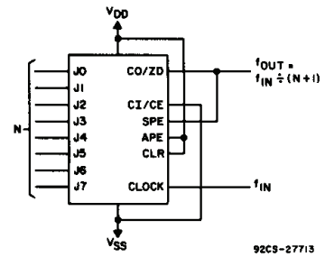
Fig. 18 - Divide-by-"N" counter.
