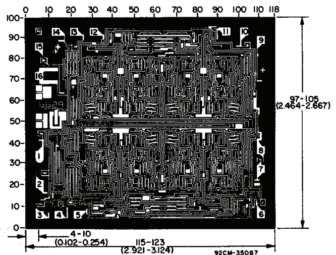
Dimensions and pad layout for CD40103B.
