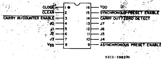
CD40102B, CD40103B TERMINAL ASSIGNMENT
