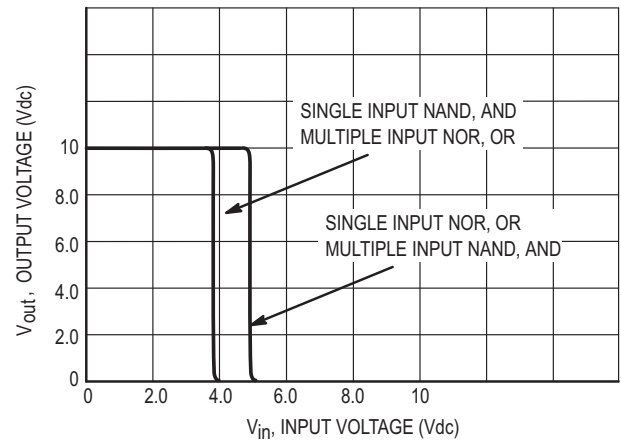
Figure 9. V_{DD} = 10 Vdc
