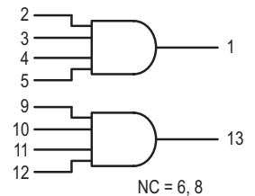
MC14082B Dual 4-Input AND Gate
