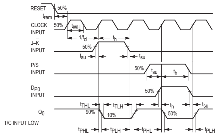
Figure 1. Timing Diagram
