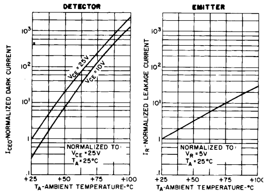
Fig. 4. Leakage Currents vs. Temperature
