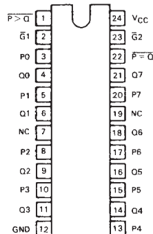
CONNECTION DIAGRAMS (TOP VIEW)
