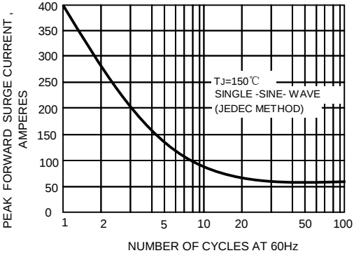
FIG.2-MAXMUN NON-REPETITIVE SURGE CURRENT
