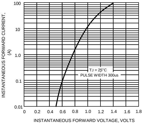
FIG.4-TYPICAL FORWARD CHARACTERISTICS
