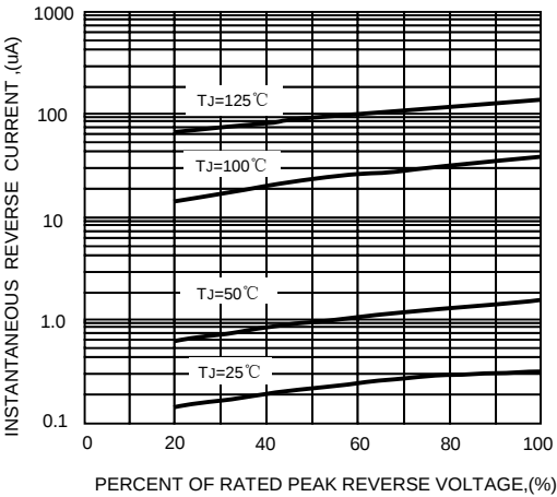
FIG.3-TYPICAL REVERSE CHARACTERISTICS
