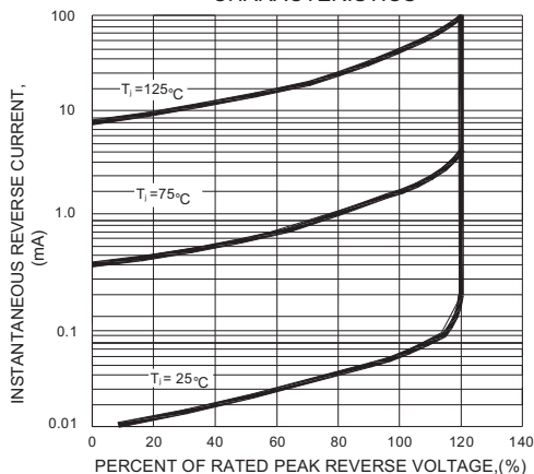
FIG.3-TYPICAL REVERSE CHARACTERISTICS
