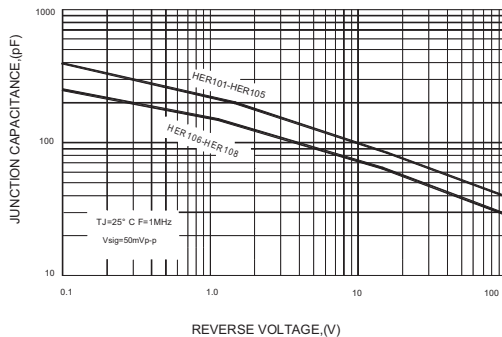
FIG.5-TYPICAL JUNCTION CAPACITANCE
