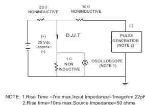
FIG.6-TEST CIRCUIT DIAGRAM REVERSE RECOVERY TIME CHARACTERISTIC
