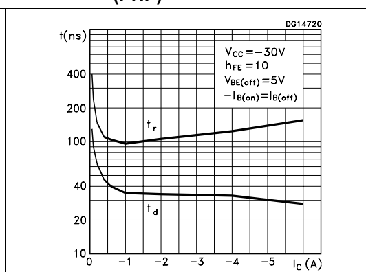
Figure 13. Resistive load switching time (PNP)
