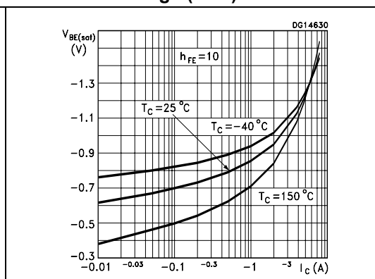
Figure 11. Base-emitter voltage (PNP)
