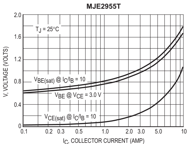
Figure 4. "On" Voltages
