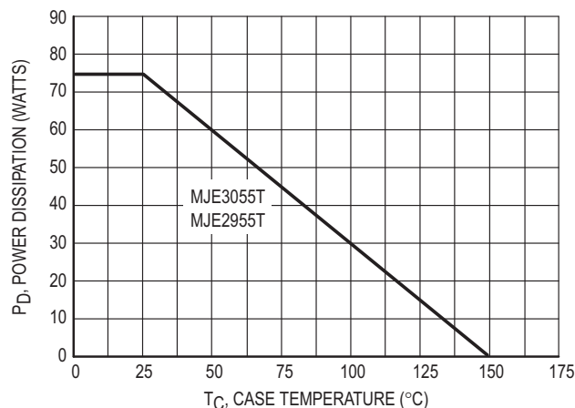
Figure 3. Power Derating
