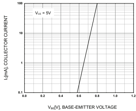
Figure 2. Transfer Characteristic
