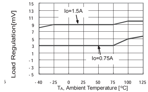
Figure 2. Load Regulation
