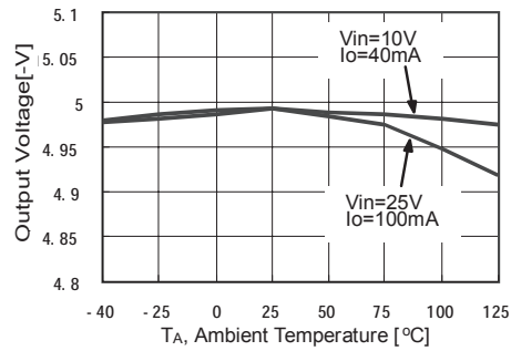
Figure 1. Output Voltage
