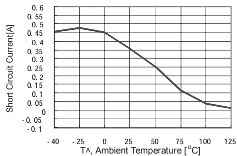
Figure 5. Short Circuit Current
