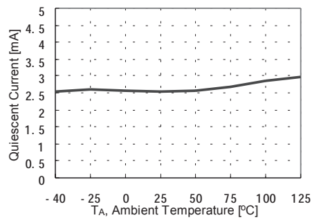
Figure 3. Quiescent Current
