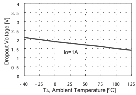
Figure 4. Dropout Voltage
