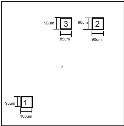
Pad Location 78L06
