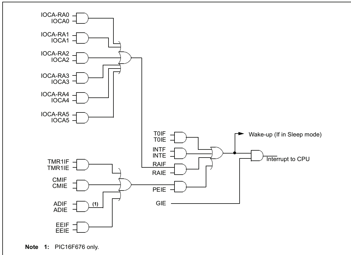
FIGURE 9-10: INTERRUPT LOGIC
