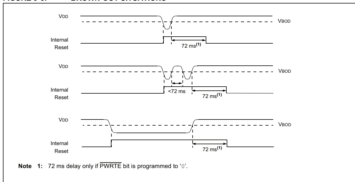
FIGURE 9-6: BROWN-OUT SITUATIONS
