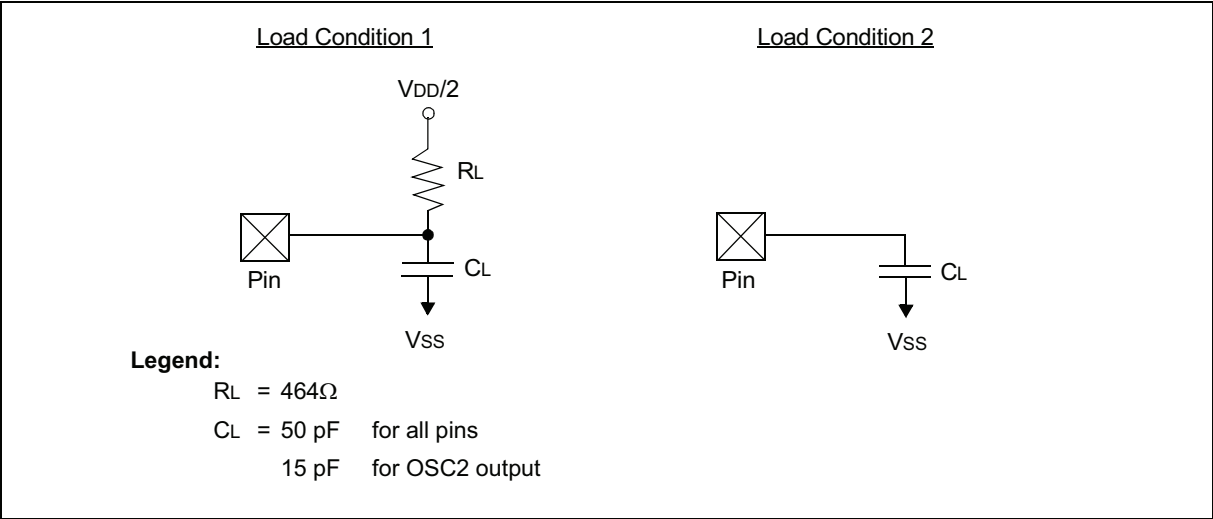
FIGURE 12-4: LOAD CONDITIONS
