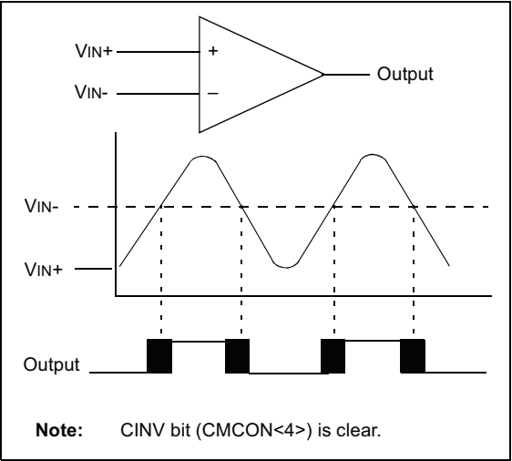
FIGURE 6-1: SINGLE COMPARATOR
