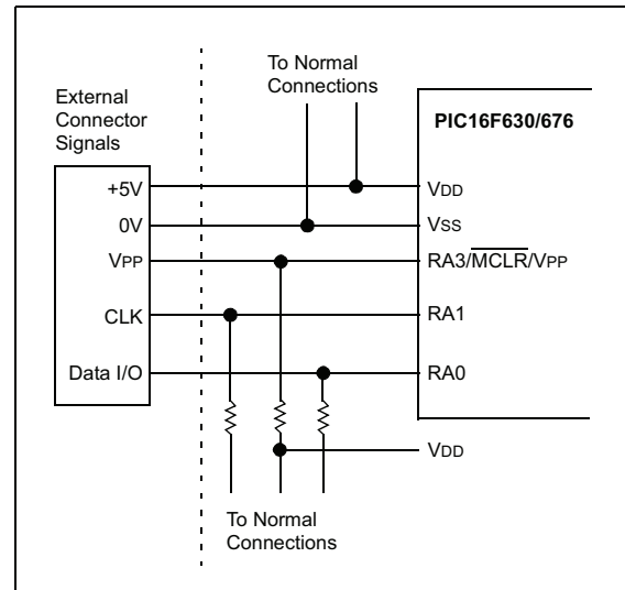
FIGURE 9-14: TYPICAL IN-CIRCUIT SERIAL PROGRAMMING CONNECTION
