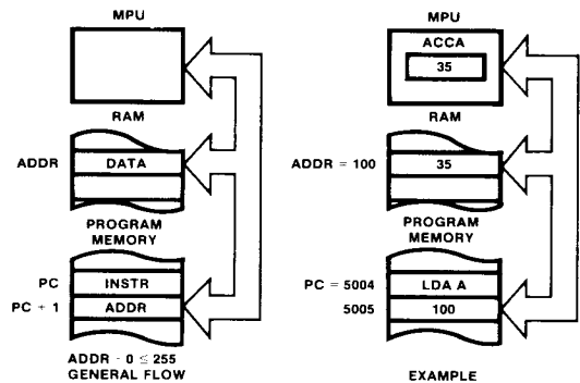
Fig. 23 Direct Addressing Mode
