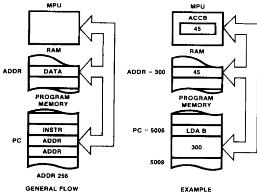
Fig. 24 Extended Addressing Mode
