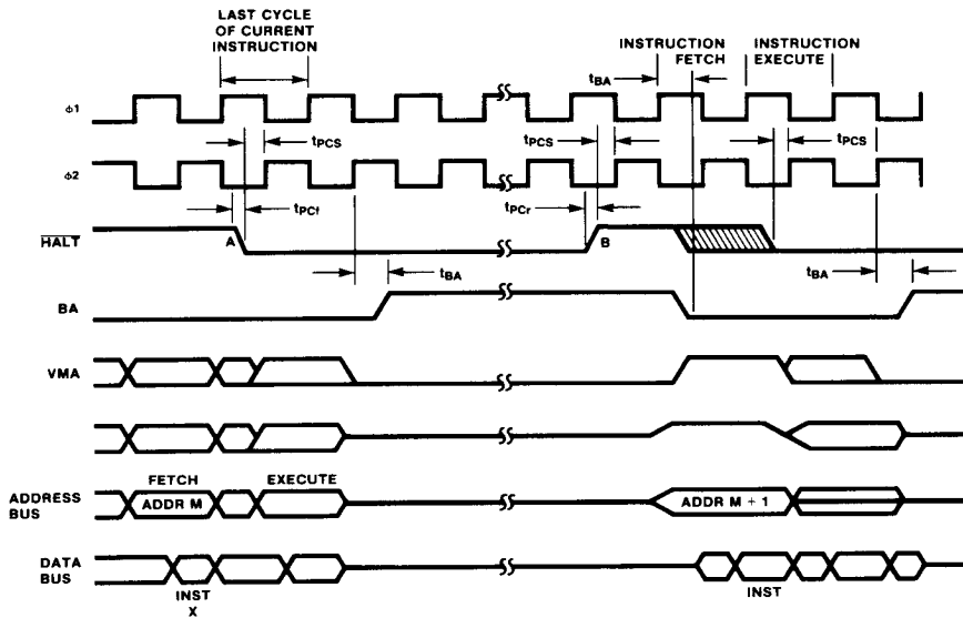
Fig. 6 Halt and Single Instruction Execution for System Debug
