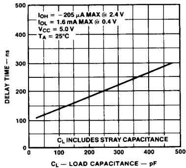
Fig. 30 Typical Data Bus Output Delay vs Capacitive Loading ( t_{ODW} )
