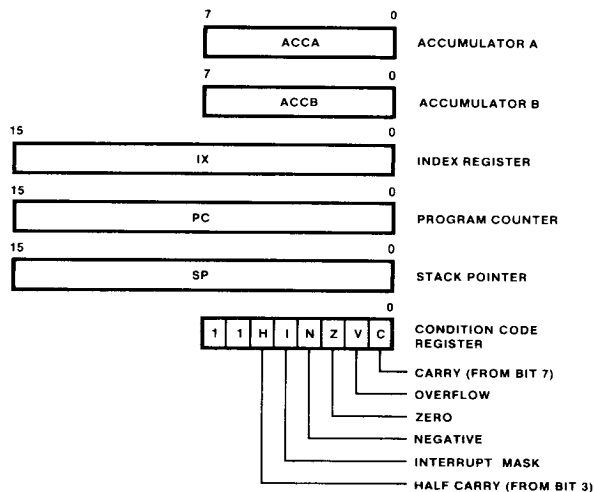
Fig. 7 Programming Model of The Microprocessing Unit
