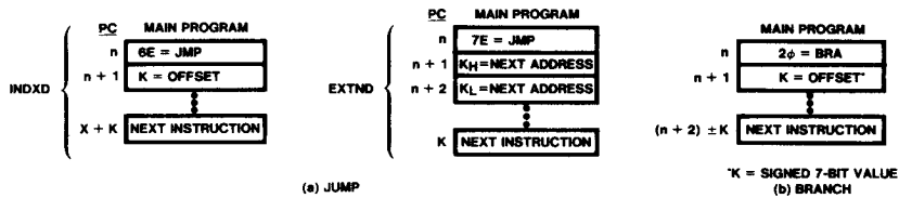
Fig. 10 Program Flow for Jump and Branch Instructions
