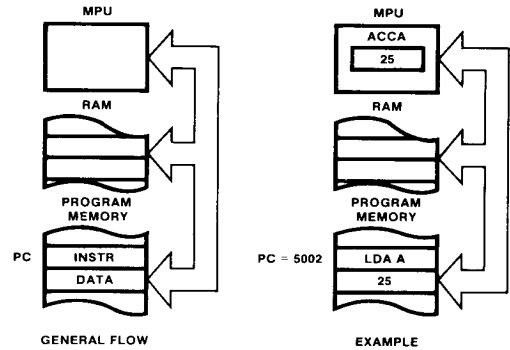
Fig. 22 Immediate Addressing Mode
