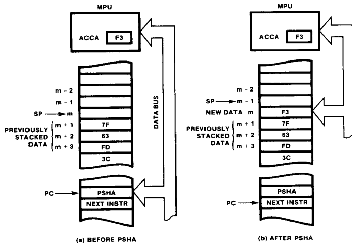
Fig. 8 Stack Operation, Push Instruction
