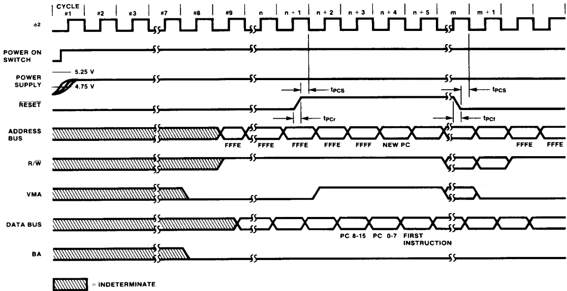
Fig. 2 Reset Timing
