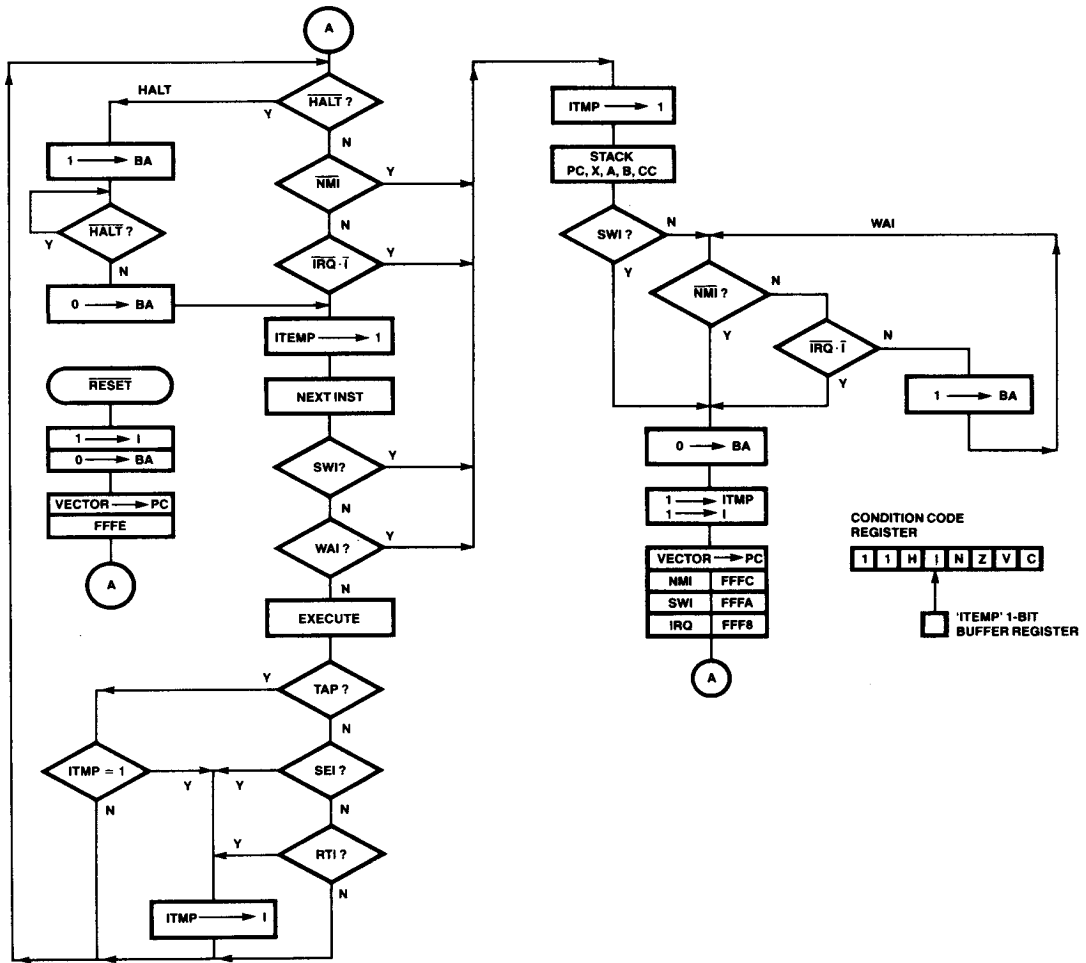
Fig. 1 MPU Flow Chart
