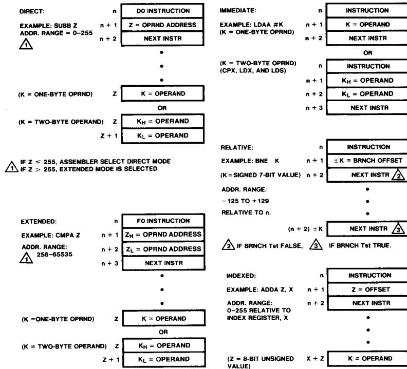
Fig. 19 Addressing Mode Summary
