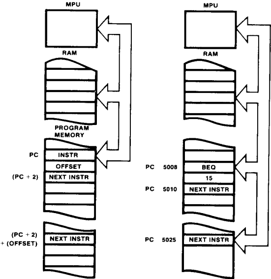
Fig. 25 Relative Addressing Mode
