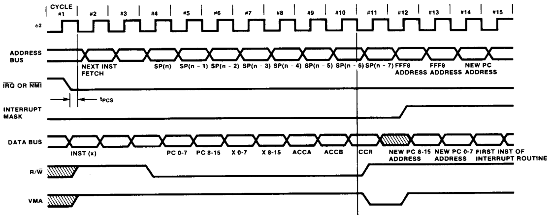
Fig. 3 Interrupt Timing
