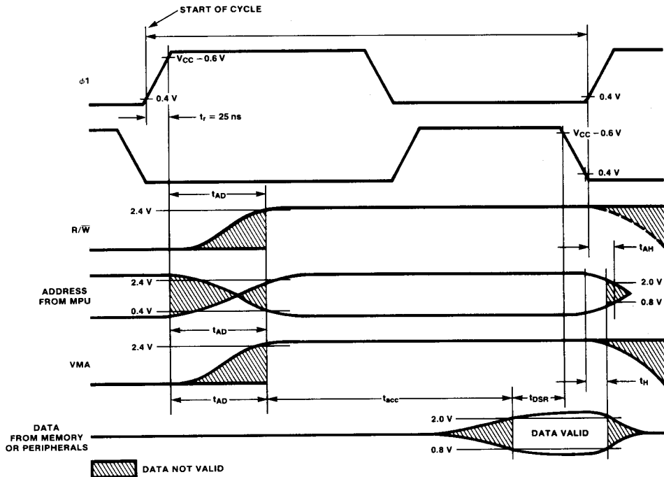
Fig. 28 Read Data From Memory or Peripherals
