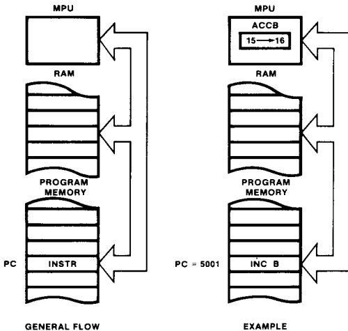
Fig. 21 Accumulator Addressing
