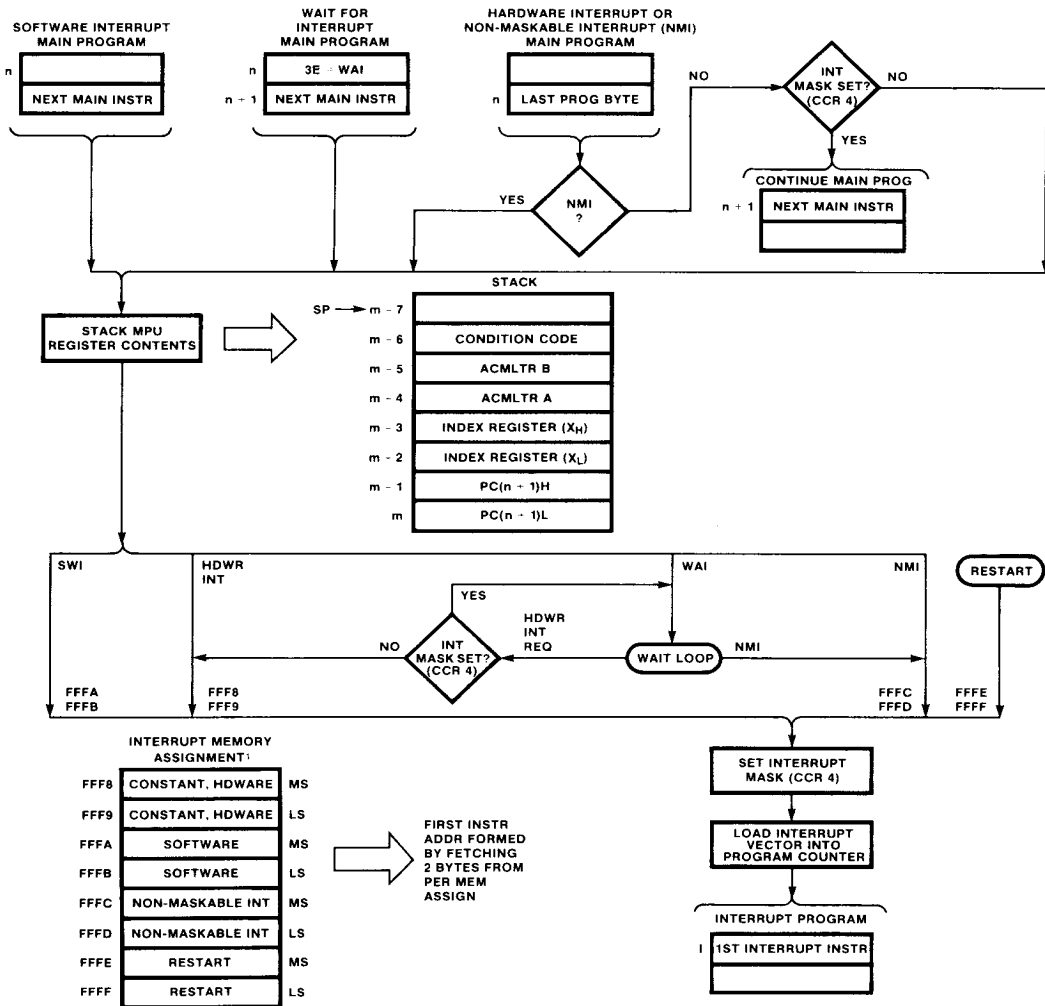
Fig. 16 Program Flow for Interrupts
