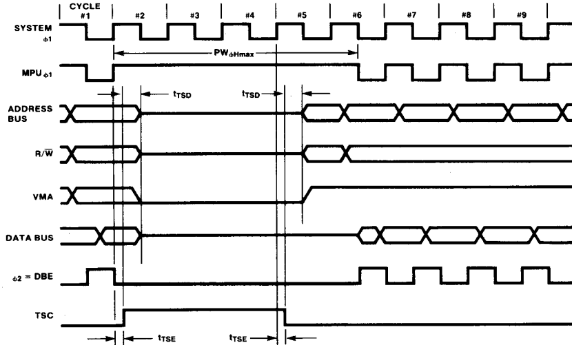
Fig. 5 3-State Control Timing
