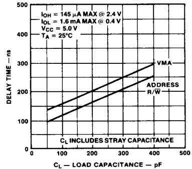
Fig. 31 Typical READ/WRITE, VMA, and Address Output Delay vs Capacitive Loading ( t_{AD} )
