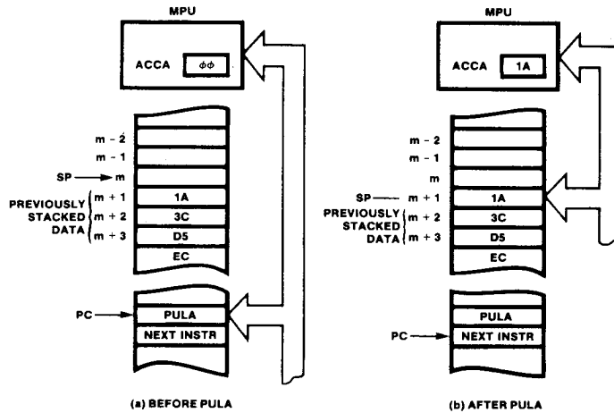
Fig. 9 Stack Operation, Pull Instruction
