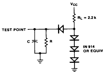
Fig. 32 Bus Timing Test Loads
