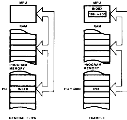
Fig. 20 Inherent Addressing
