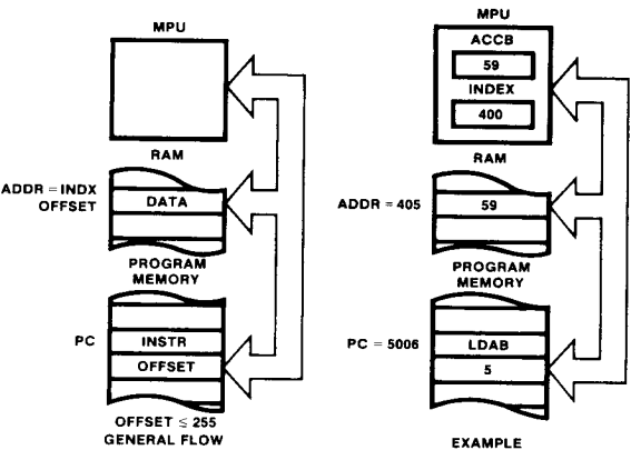
Fig. 26 Indexed Addressing Mode
