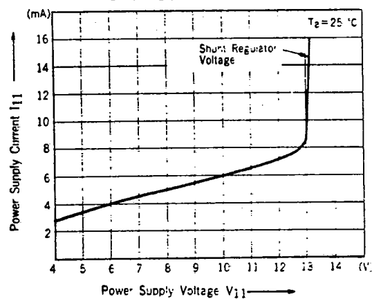
POWER SUPPLY CURRENT vs. POWER SUPPLY VOLTAGE
