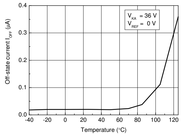
Figure 16. Off-state cathode current vs. temperature
