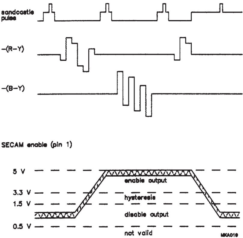
Fig.4 Timing waveforms.
