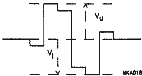
Fig.3 Non-linearity definition.
