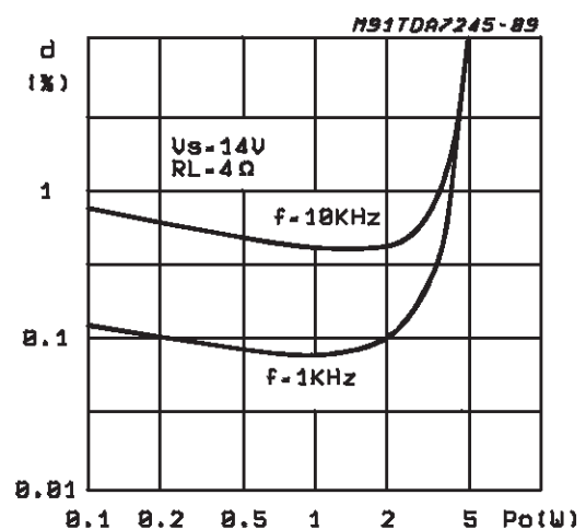
Figure 9: Distortion vs. Output Power
