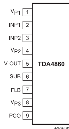
Fig.2 Pin configuration.
