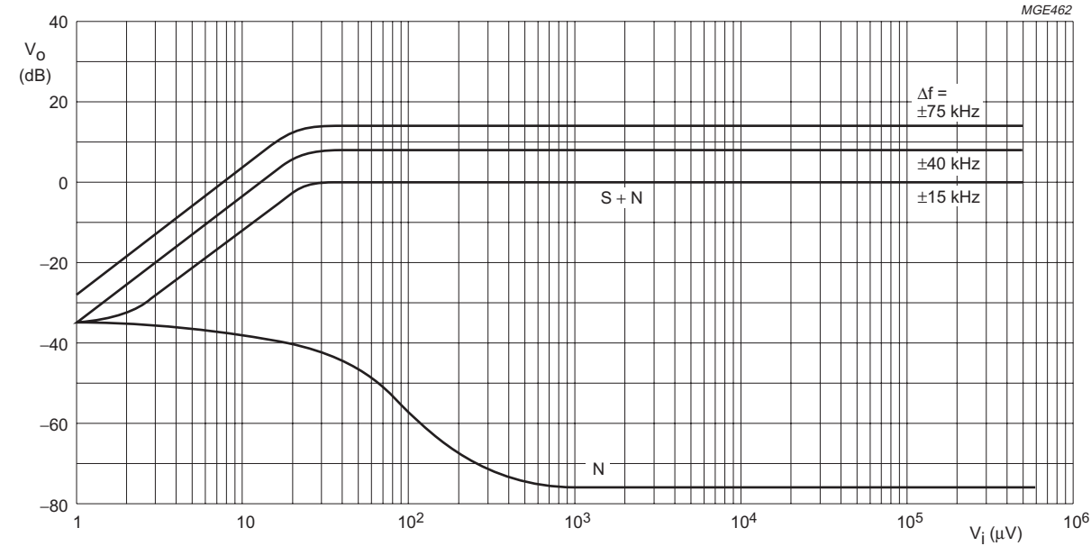
Fig.6 AF output voltage level as a function of IF input voltage; V_p = 15 V; f_m = 400 Hz; B = 250 Hz to 16 kHz; Q_L = 20 ; C_{8-9} = 6.8 nF.
