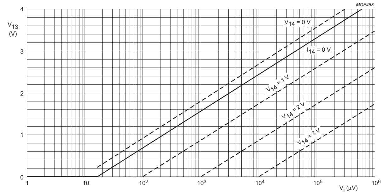
Fig.7 Voltage at field strength indicator output (proportional to V_{12} ); R_{13} = 3.6 k \Omega .
