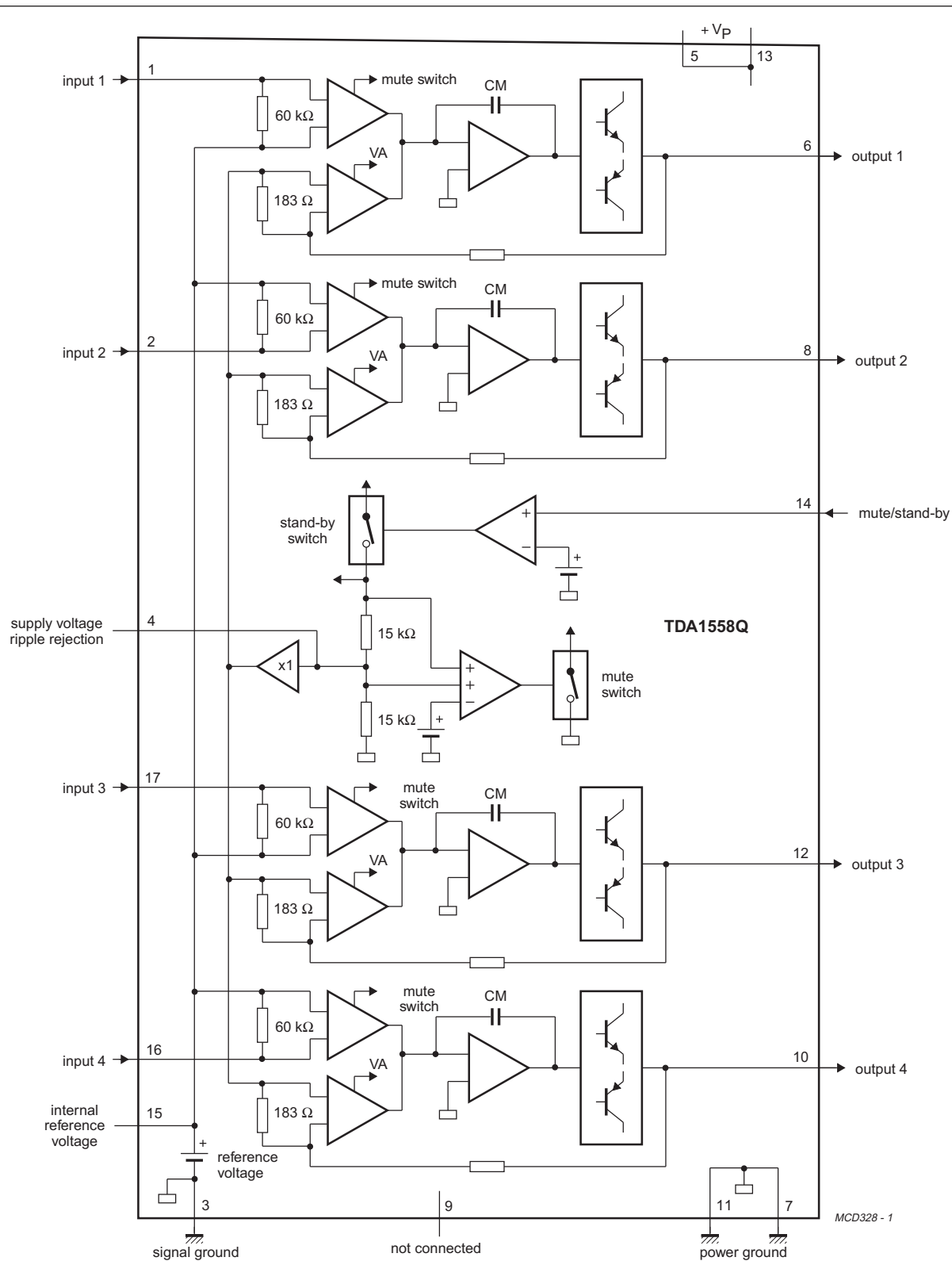
Fig.1 Block diagram.
