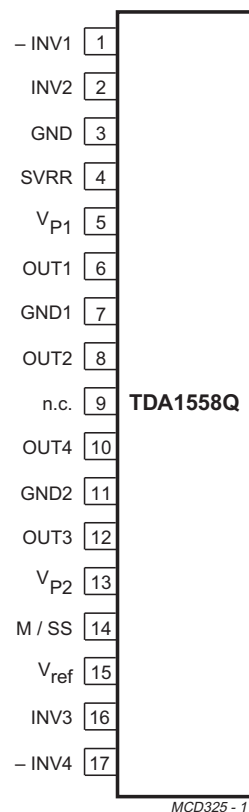
Fig.2 Pin configuration.
