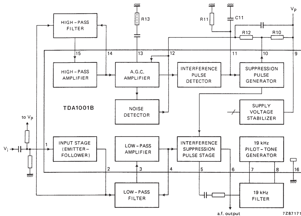
Fig.1 Block diagram.
