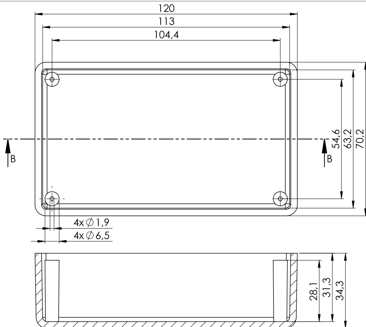
SECTION B-B
