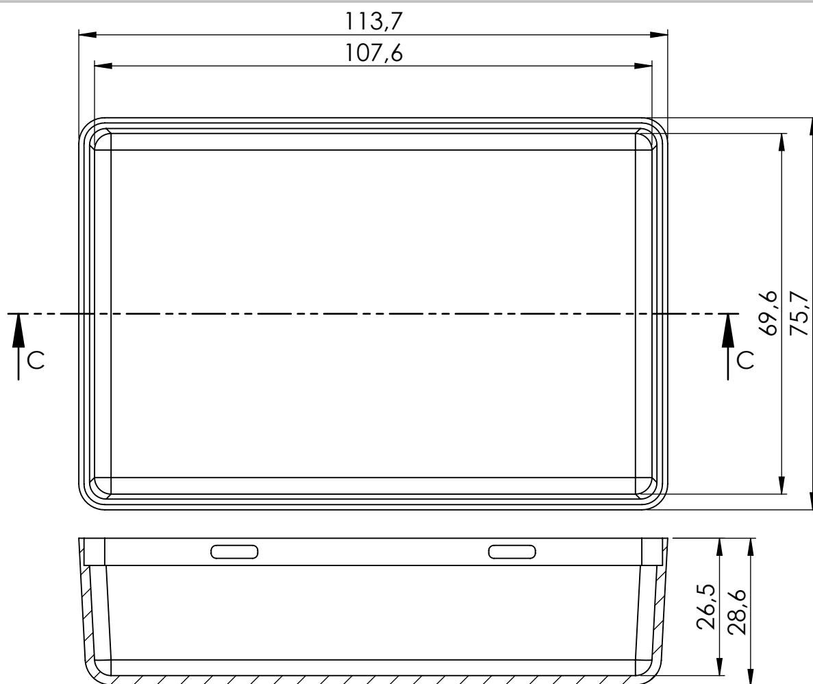
SECTION C-C
