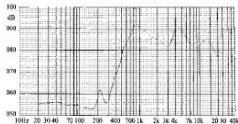
FREQUENCY RESPONSE [actual curve of type]
