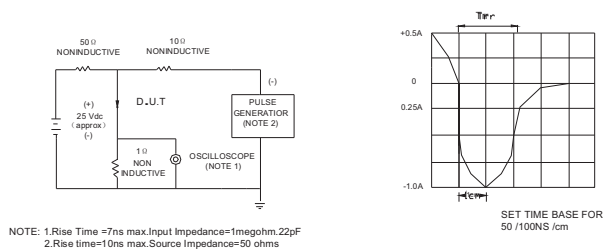
FIG.6-TEST CIRCUIT AND TYPICAL REVERSE RECOVERY TIME CHARACTERISTIC
