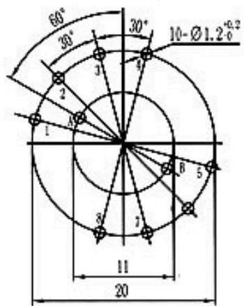
P. B. C. MOUNTING HOLE DETAIL
