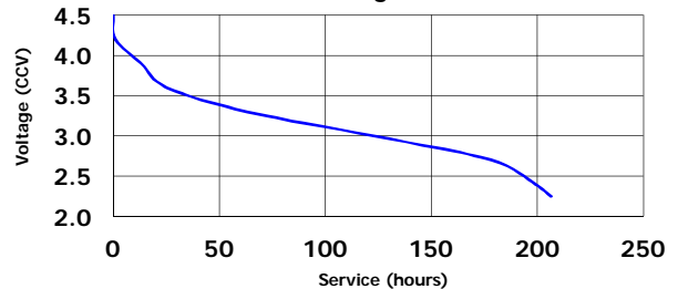
3.9 ohm Continuous Discharge
