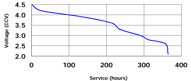
RADIO 220 ohm 4 hrs/day
