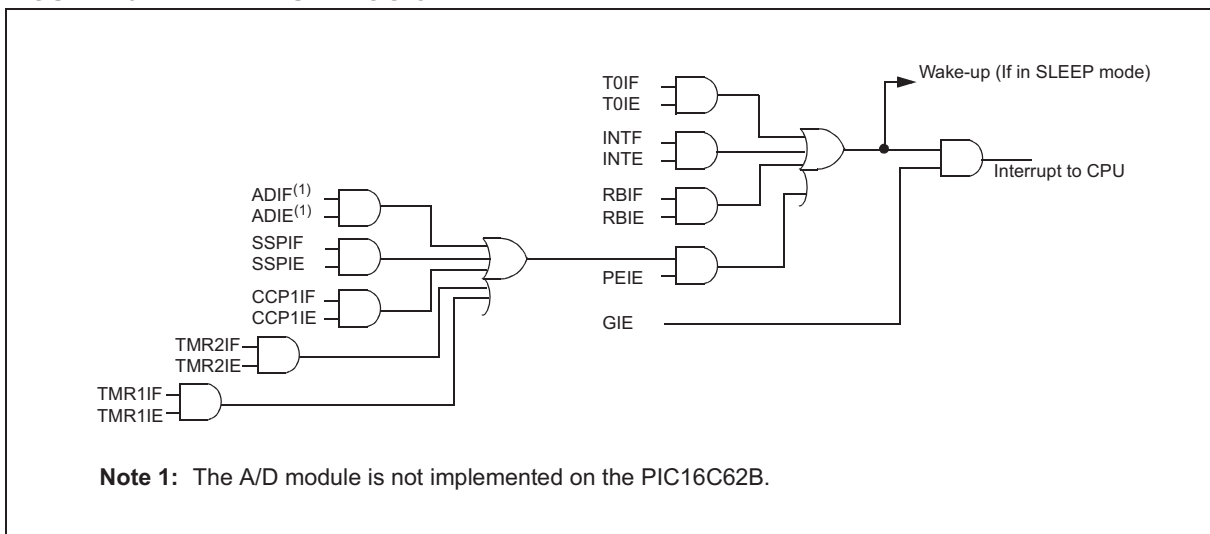
FIGURE 10-7: INTERRUPT LOGIC
