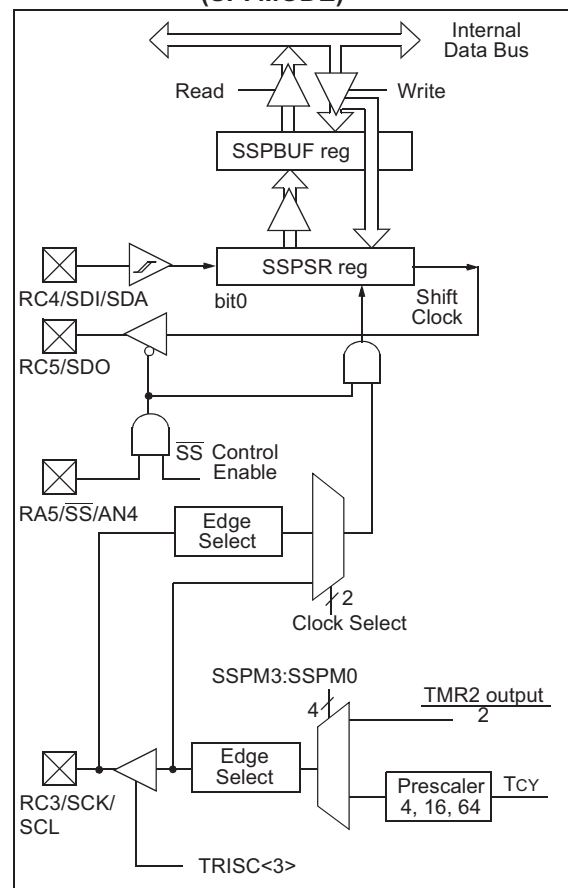
FIGURE 8-1: SSP BLOCK DIAGRAM (SPI MODE)
