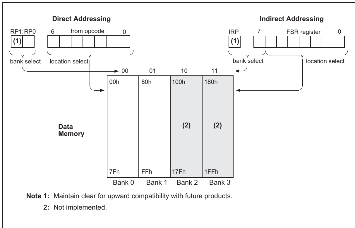
FIGURE 2-3: DIRECT/INDIRECT ADDRESSING
