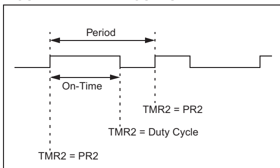
FIGURE 7-4: PWM OUTPUT
