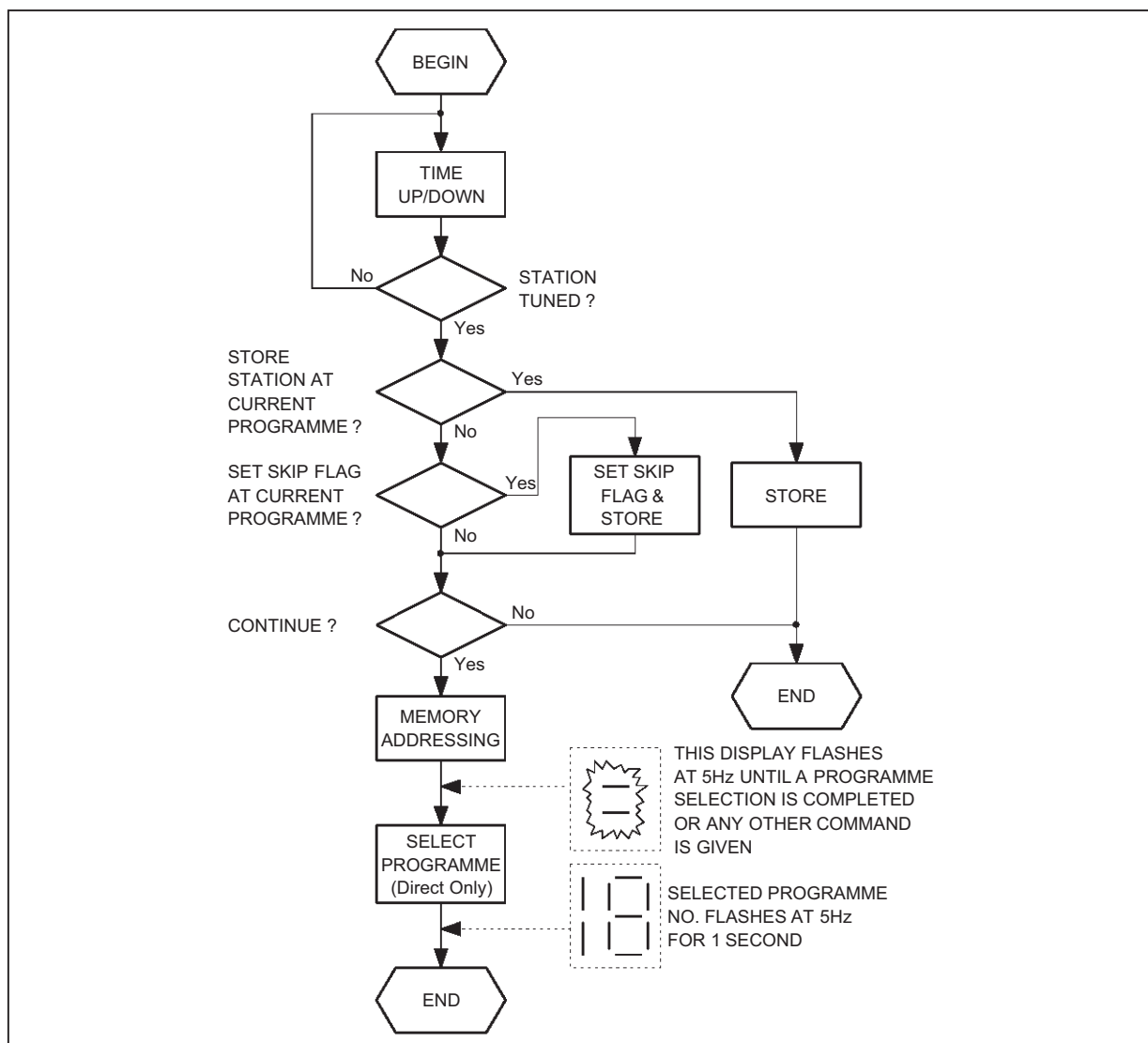
Figure 13 : Program Selection Routine (16 program)
