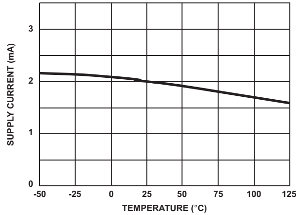
FIGURE 8. SUPPLY CURRENT vs AMBIENT TEMPERATURE
