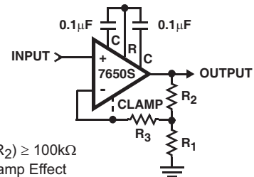
FIGURE 2. NON INVERTING AMPLIFIER WITH OPTIONAL CLAMP
