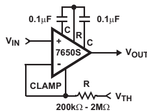
FIGURE 5. LOW OFFSET COMPARATOR
