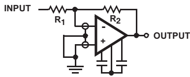
FIGURE 1A. INVERTING AMPLIFIER
