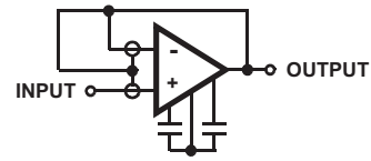
FIGURE 1B. FOLLOWER
