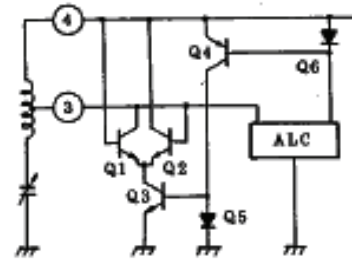
Fig.1 AM OSCILLATION CIRCUIT
