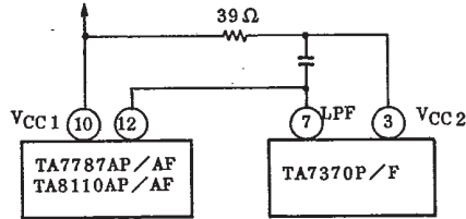
Fig.4 CONNECTION TO TA7343AP/AF AND TA7370P/F
