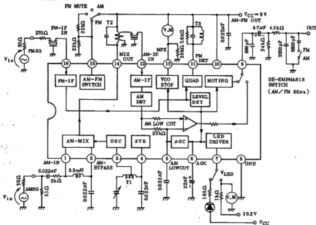
TEST CIRCUIT 1
