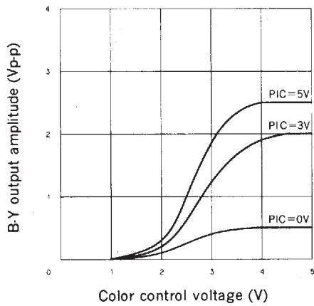
Color Control Characteristics (When color bar is input)
