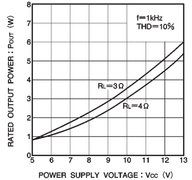
Fig. 11 Output power vs. power supply voltage
