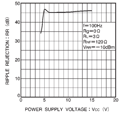
Fig. 17 Ripple rejection ratio vs. power supply voltage
