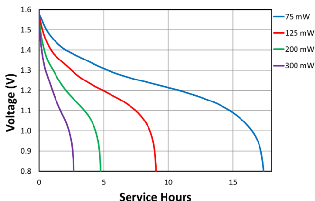
Constant Power
