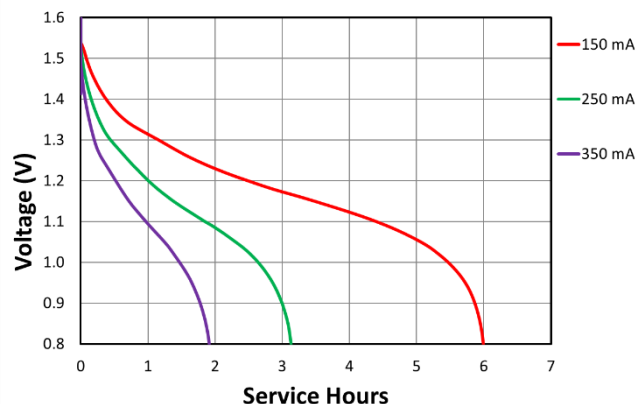
Constant Current
