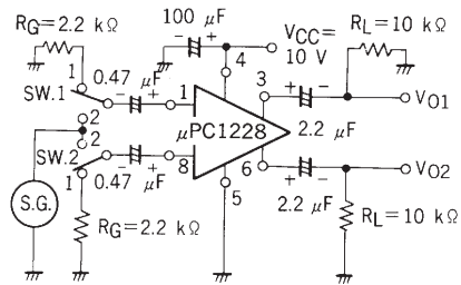
(4) Cross talk, Channel balance test circuit
