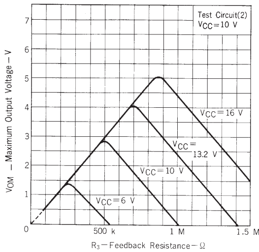
MAXIMUM OUTPUT VOLTAGE vs. FEEDBACK RESISTANCE
